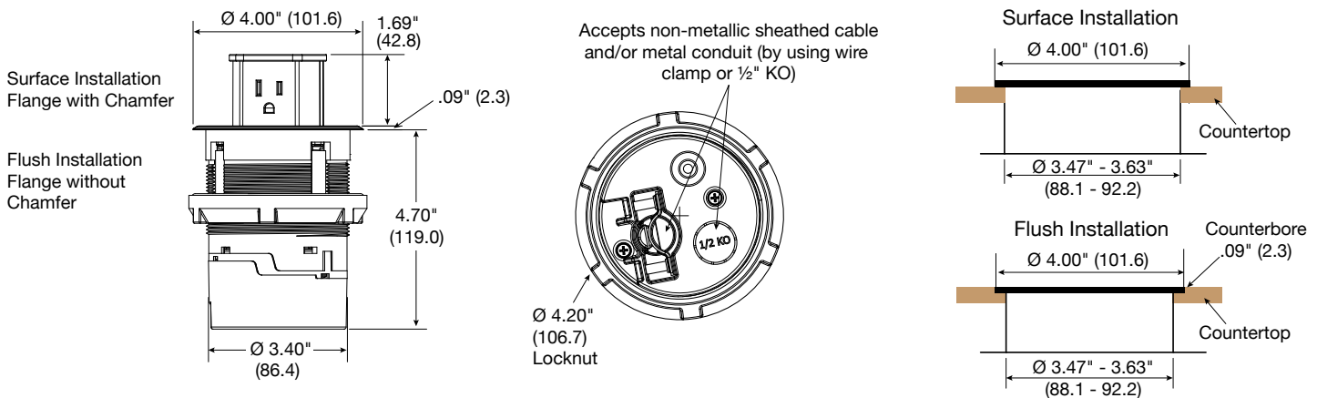
Flush Mount
